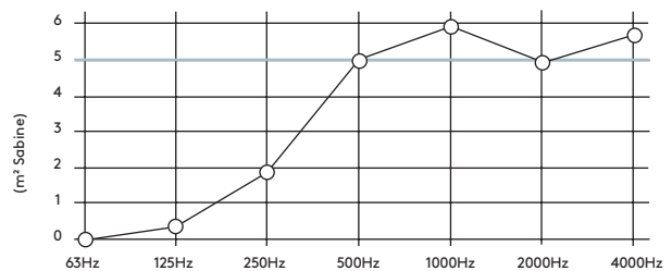
Equivalent Sound Absorption Area (m 2 Sabine)/Unit*
