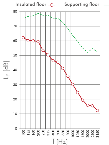
Insulation against impact noise - BBRI test report AC 7994
